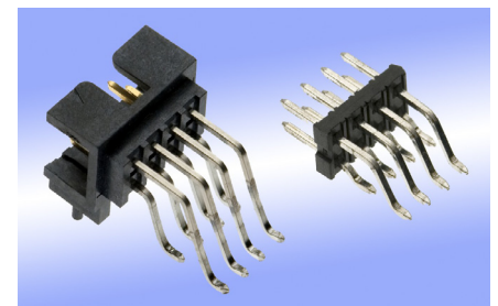
Milli-Grid™ Shrouded (Series 78264) and Unshrouded Custom Headers (Series 87979) with Horizontal SMT solder tails
