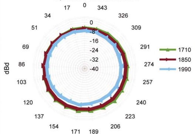
estimated gain (dBd) 1800/1900 MHz band
