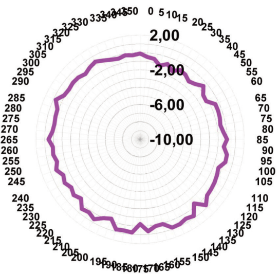
Freq. 1800 MHz H-plane (dBi) V-pol
