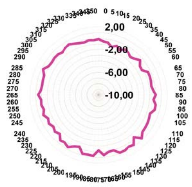
Freq. 1800 MHz H-plane (dBi) V-pol
