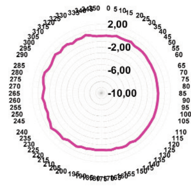
Freq. 1800 MHz H-plane (dBi) V-pol
