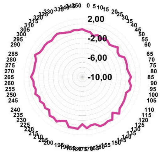
Freq. 1800 MHz H-plane (dBi) V-pol
