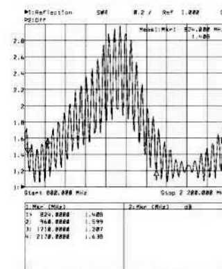
SWR CURVE
