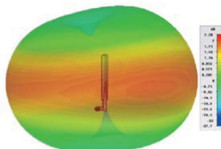
Typical 3D Plot (1800 MHz)
